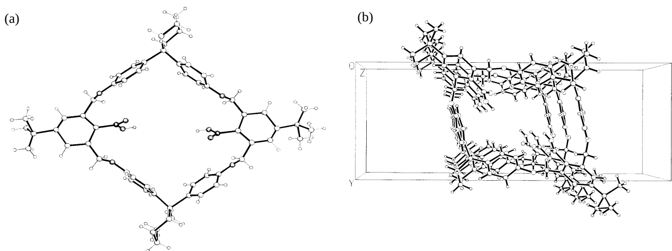
Fig. 3 X-ray crystal structure of 5',28'-Di- tert -butyl-1',10',24',33'-tetraoxa-dispiro[cyclohexane-1,17'-([2](1,3)benzeno[2](1,4)benzeno[1](1,4)benzeno[2](1,3)benzeno[2](1,4)benzeno[1](1,4)benzenophane)-40',1"-cyclohexane]-8',31'-dicarboxylic acid ( 1 )·2 EtOH: (a) Molecular plot (guest molecules were not determined); (b) excerpt of the packing structure showing the channel formation.
