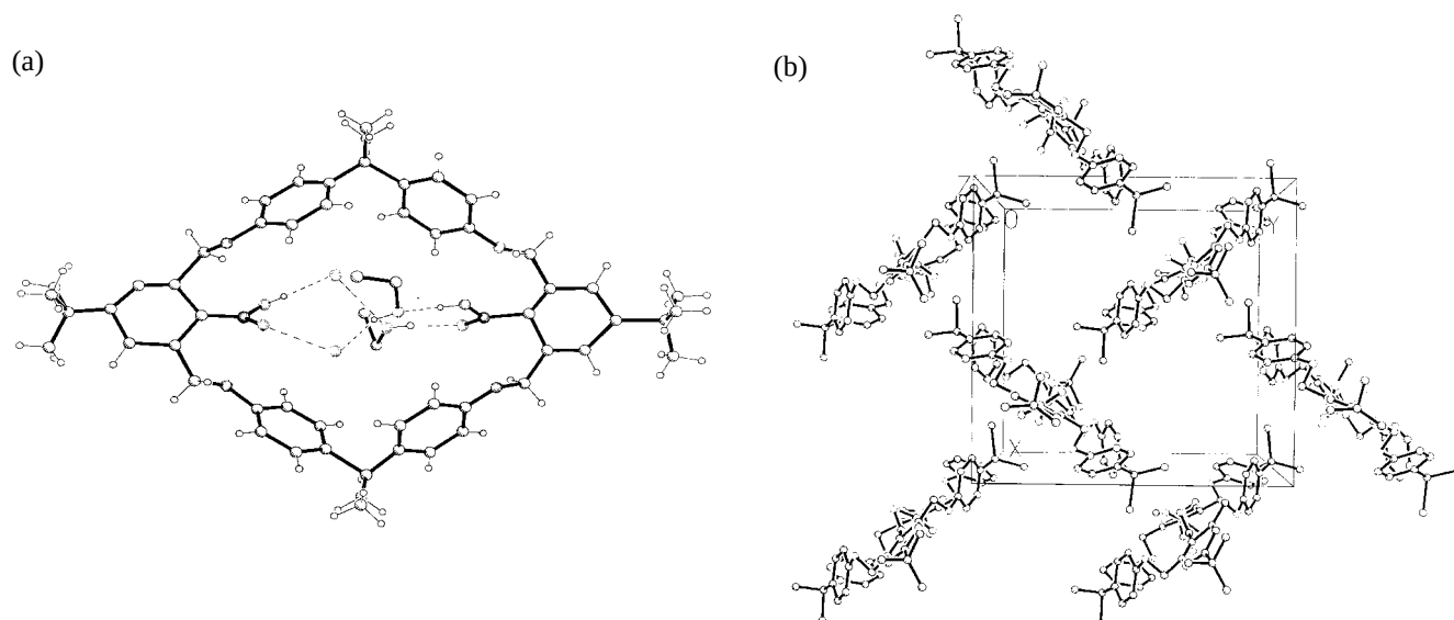
Fig. 4 X-ray crystal structure of 5,28-Di- tert -butyl-17,17,40,40-tetramethyl-1,10,24,33-tetraoxa-[2](1,3)benzeno[2](1,4)benzeno[1](1,4)benzeno[2](1,3)benzeno[2](1,4)benzeno[1](1,4)benzenophane-8,31-dicarboxylic acid ( 2 )·2 EtOH·2 H 2 O: (a) Molecular plot; (b) packing structure (guest molecules are omitted).
